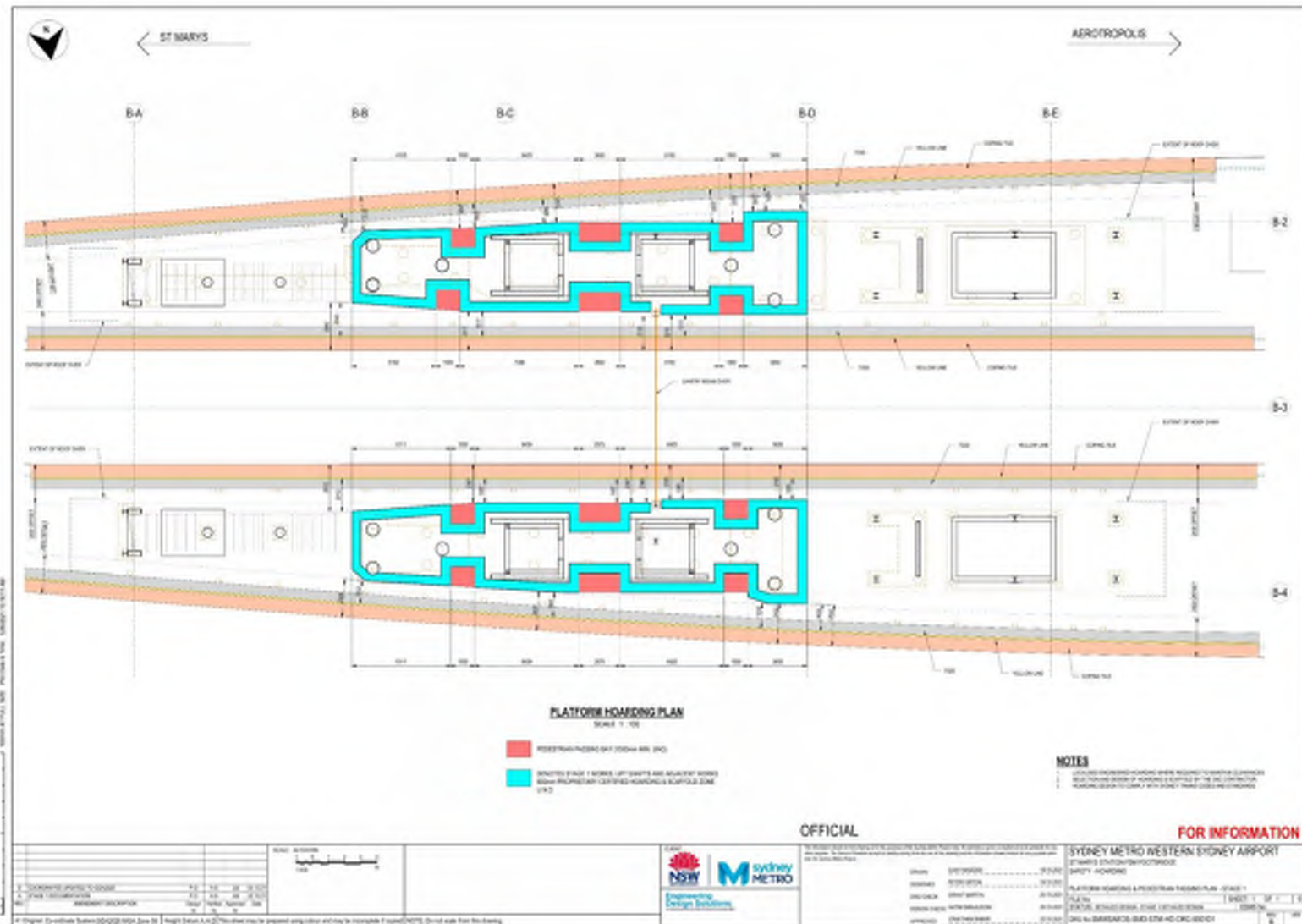
Figure 7: Preliminary platform hoarding plan for Stage 1 of the FSM works (Engineering Design Solutions 2022)
